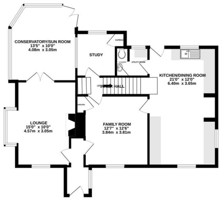
GROUND FLOOR 864 sq.ft. (80.3 sq.m.) approx.
