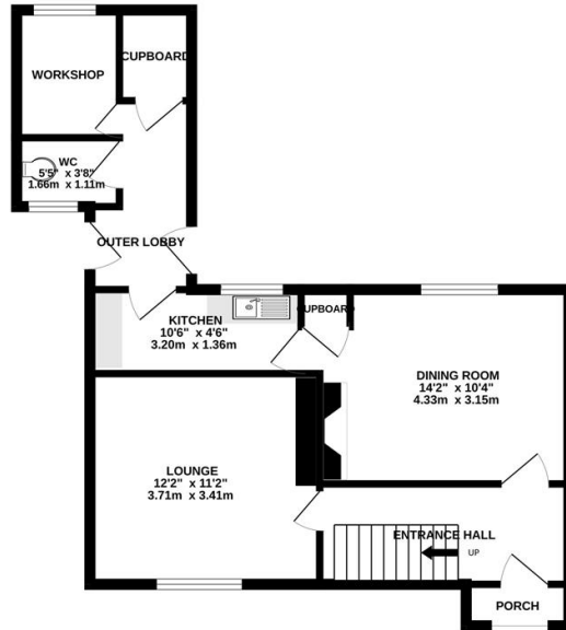
GROUND FLOOR 517 sq.ft. (48.1 sq.m.) approx.
